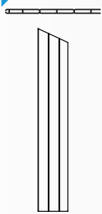
Privacy Board 4 (1) ½" x 10⅝" x 65⅞"
